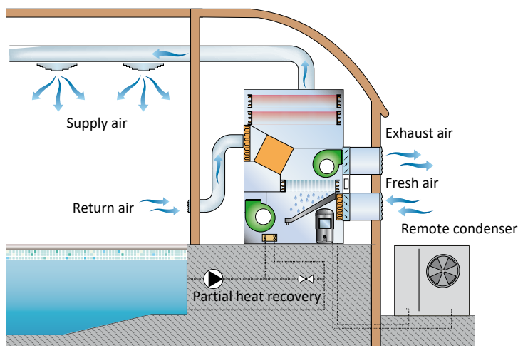
Plant scheme with UTAZ
